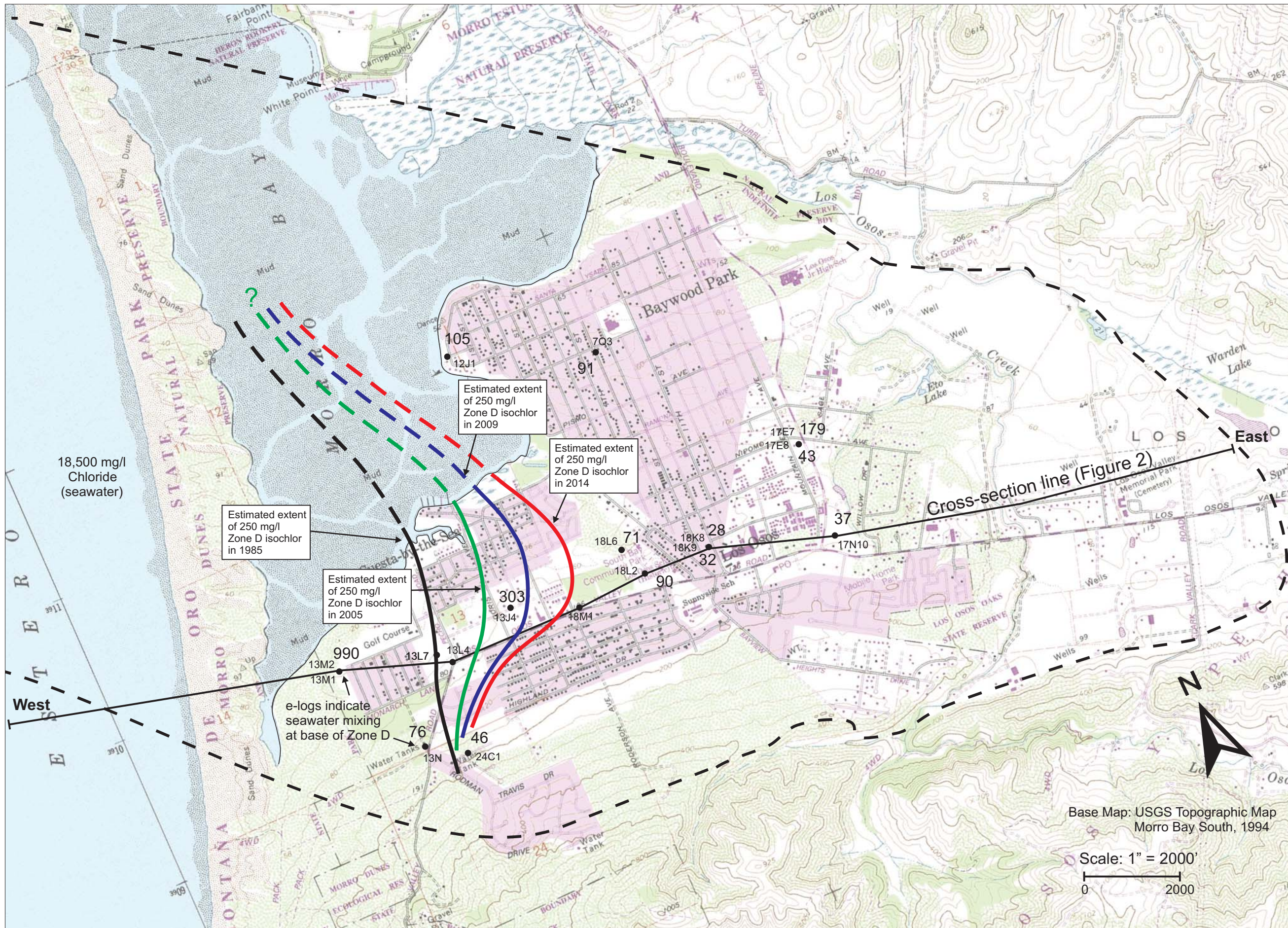
Figure 1 Lower Aquifer Chloride Concentrations and Zone D Intrusion Front Seawater Intrusion 2014 Update Los Osos ISJ Cleath-Harris Geologists
